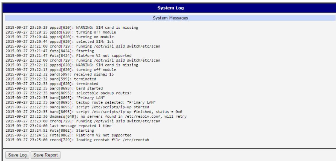
Figure 4: System Log
