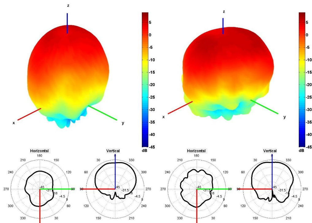
3350 and 3600 MHz Radiation pattern
