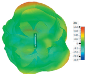
3D Plot Element A Side (5400MHz)
