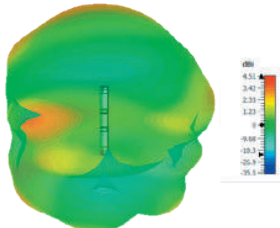
3D Plot Element A Top (2600MHz)
