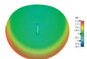
3D Plot Element D Side (1800 MHz)
