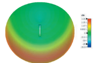
3D Plot Element D Side (850 MHz)
