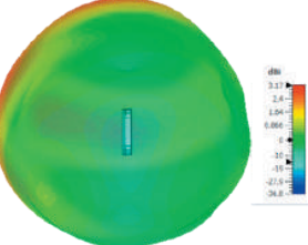
3D Plot Element A Side (2600MHz)
