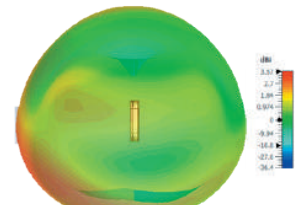
3D Plot Element D Side (2000 MHz)
