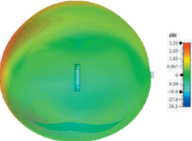
3D Plot Element A Side (2000MHz)
