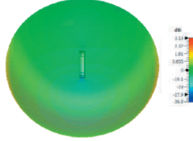
3D Plot Element A Side (850 MHz)
