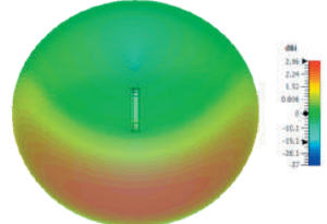
3D Plot Element D Side (750 MHz)
