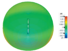
3D Plot Element D Top (750 MHz)
