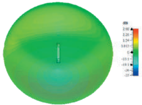
3D Plot Element A Side (750 MHz)
