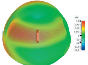
3D Plot Element D Side (2600 MHz)
