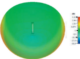
3D Plot Element A Side (1800 MHz)
