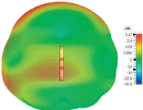
3D Plot Element A Top (2600MHz)
